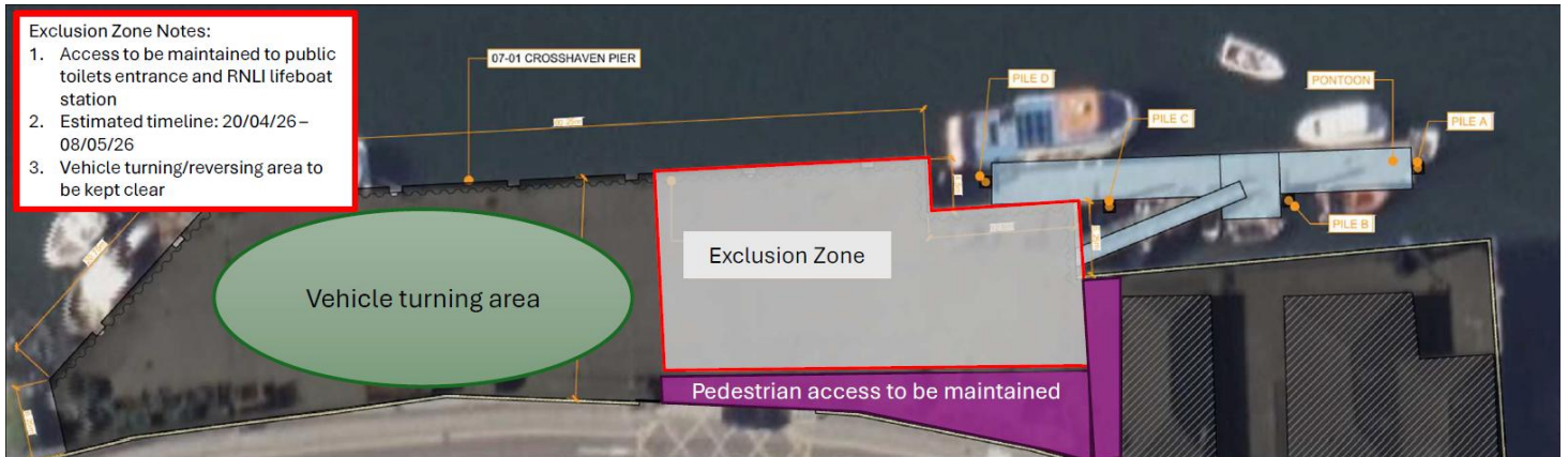
Site plan
