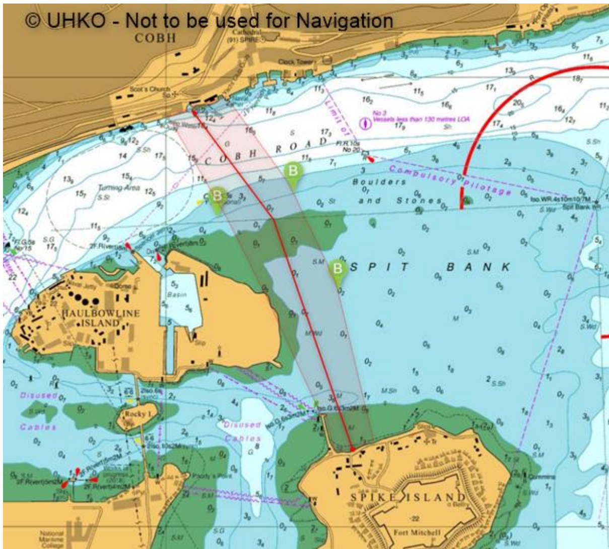
Chart 1777 (extract)
